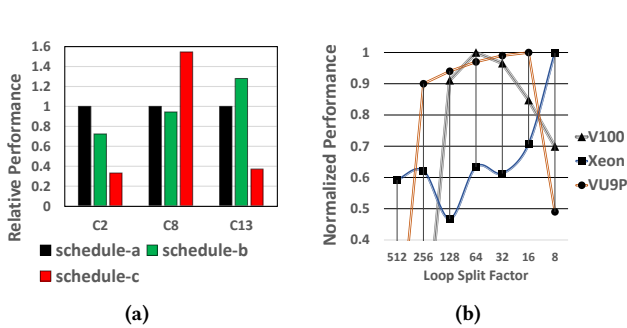
Figure 1. (a) Relative performance of three different schedules for 2D convolutions on the same platform. (b) Normalized performance of different split factors for 2D convolution on V100, Xeon E5 and VU9P.
